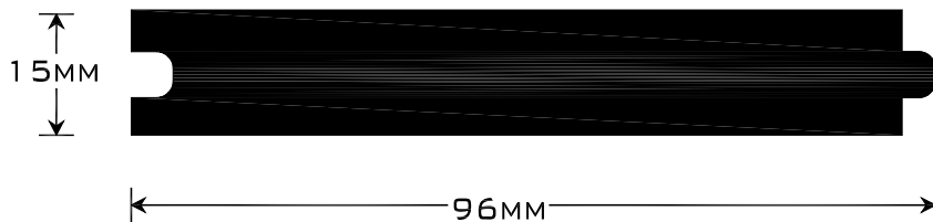
STYLEBOARD STRANDWOVEN BAMBOO FLOOR BOARD • 1830MM LENGTH (NARROW)
